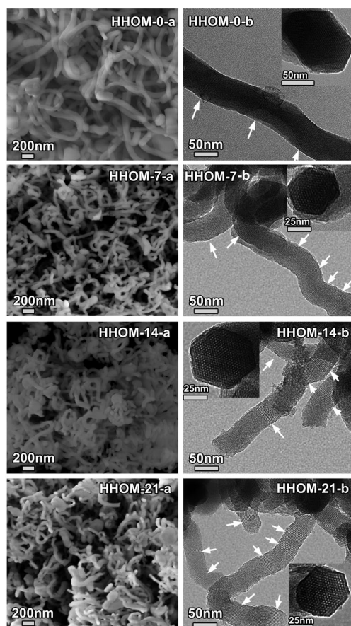
Figure 1. SEM and TEM images showing the morphology and mesostructure of the extracted samples synthesized with different molar ratios of 4 / 5 : HHOM-0 (mol % 4 = 0), HHOM-7 (mol % 4 = 7), HHOM-14 (mol % 4 = 14), and HHOM-21 (mol % 4 = 21). The arrows indicate the fringes on the images.
